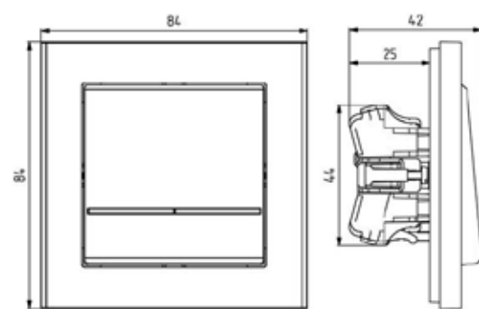
Art. no: 18 944 02/18 944 09/ 18 944 12/18 944 13
